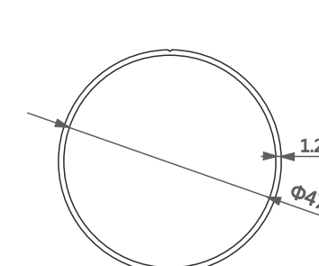
型号/Item No.-11161265-1.2 米重/Weight-0.496kg/m
