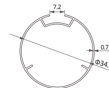
型号/Item No.-110110 米重/Weight-0.246kg/m
