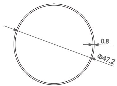
型号/Item No.-6110382-0.8 米重/Weight-0.330kg/m
