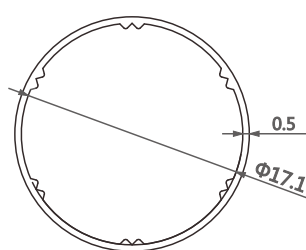
型号/Item No.-6110504 米重/Weight-0.082kg/m
