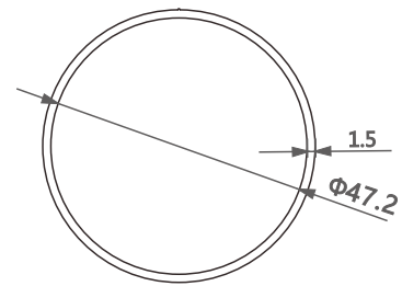
型号/Item No.-6110382 米重/Weight-0.627kg/m
